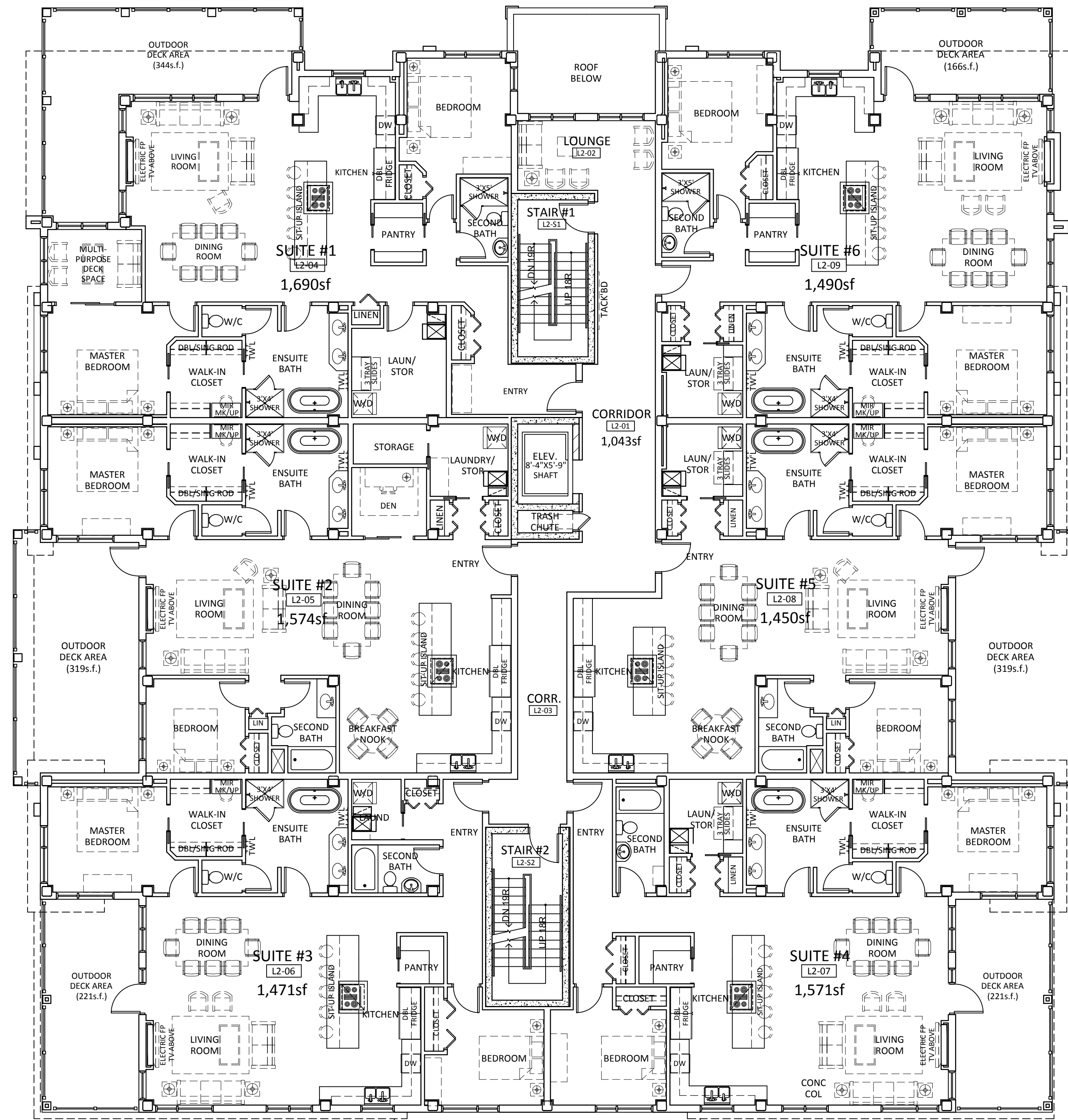
↑ N 2ND LEVEL FLOOR PLAN
