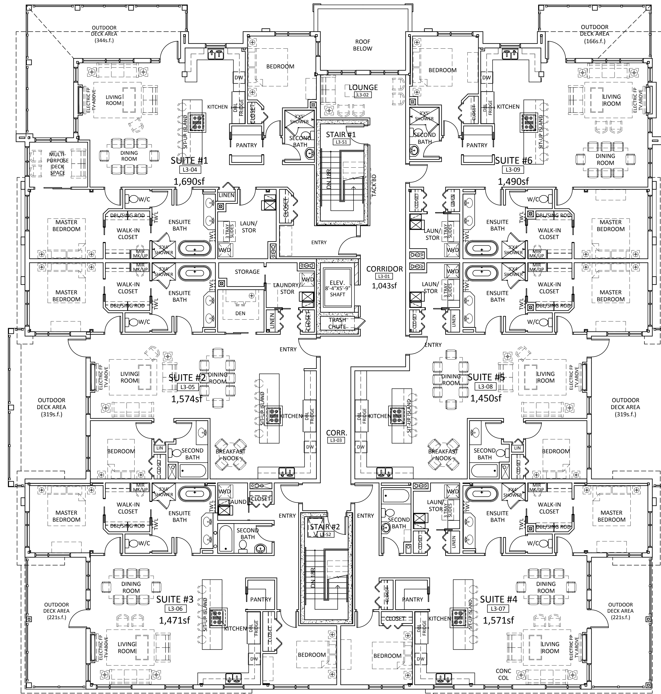
↑ N 3RD LEVEL FLOOR PLAN
